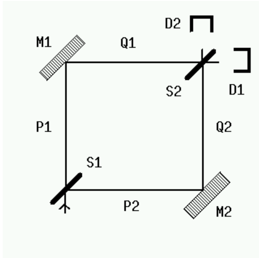
Figure 1: A simple interferometer where a particle enters as indicated and encounters a beam splitter ( S_1 ), a mirror ( M_1 or M_2 ) and a second beam splitter ( S_2 ) ending up either in detector ( D_1 ) or ( D_2 ).
